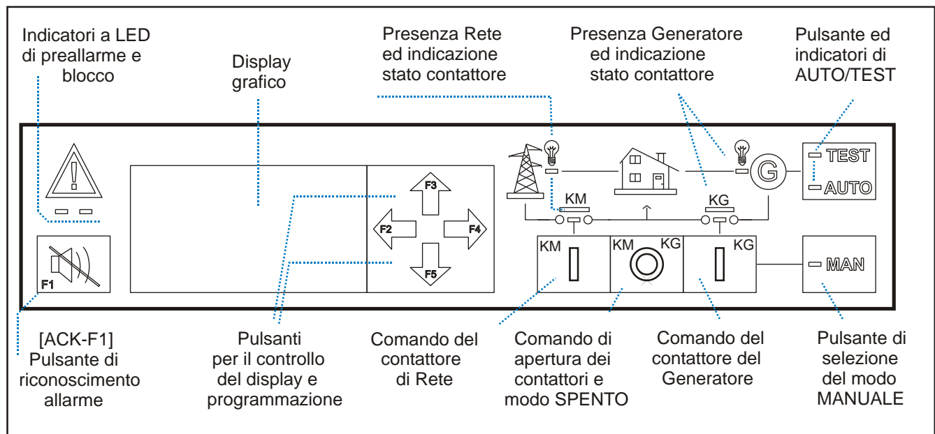
Figure 1: Pannello frontale
